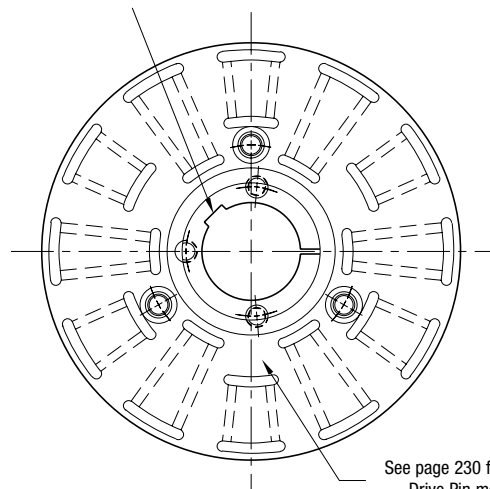
ARMATURE VIEW
