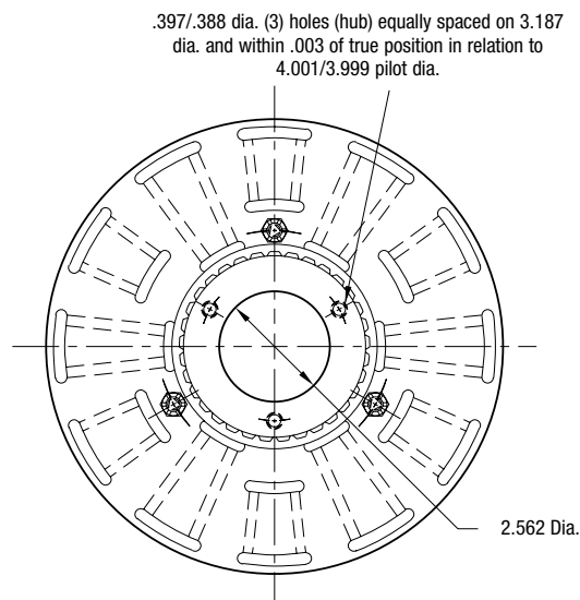
ARMATURE VIEW
