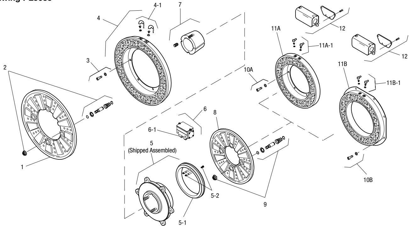
Drawing I-25635
