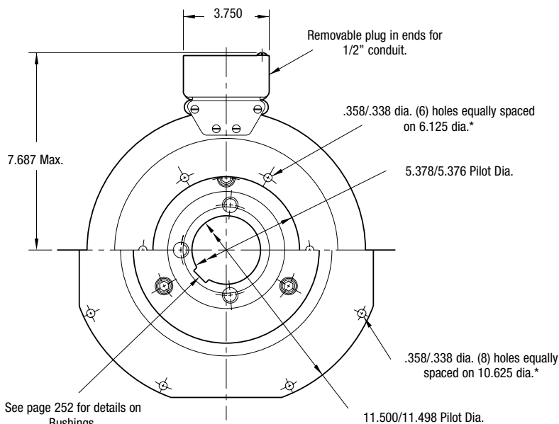
MAGNET VIEW
