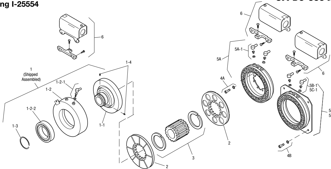
Drawing I-25554
