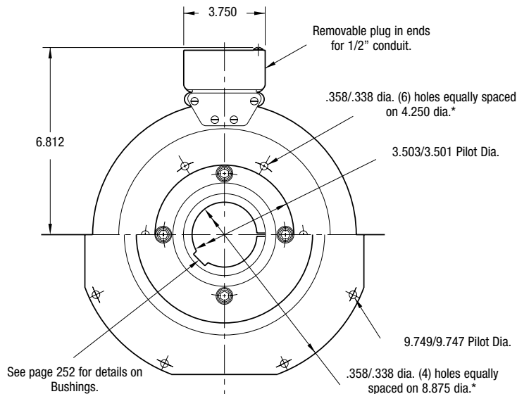
MAGNET VIEW (Inside & Outside Mounted)
