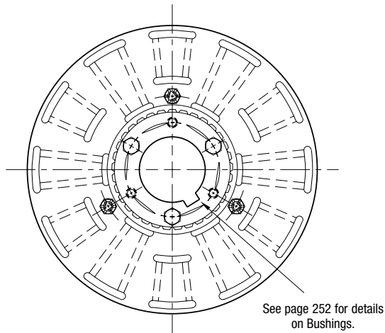
ARMATURE VIEW
