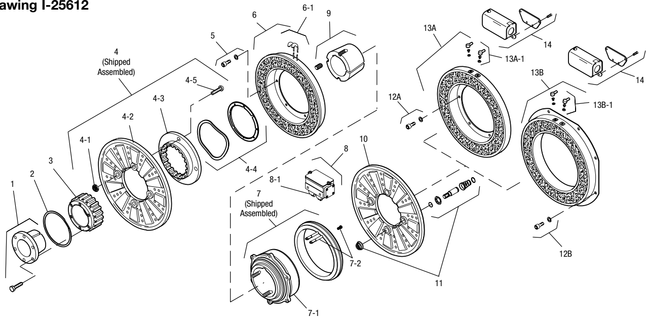
Drawing I-25612
