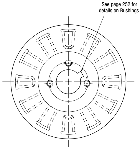
ARMATURE VIEW
