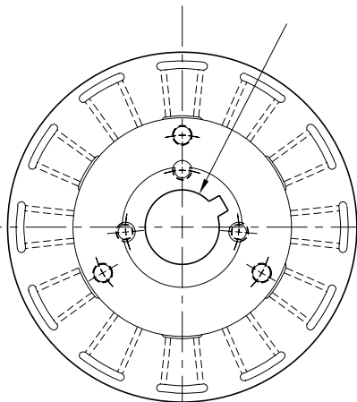
ARMATURE VIEW
