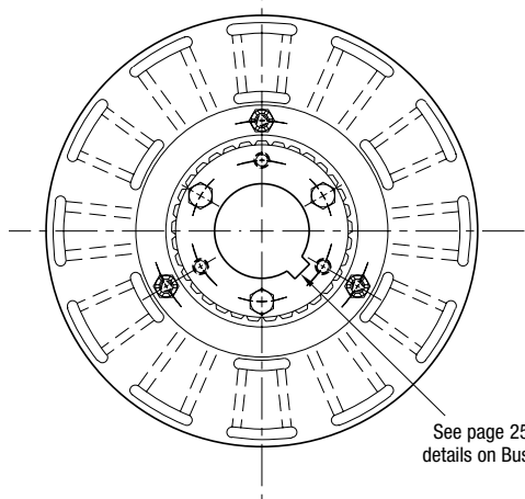
ARMATURE VIEW
