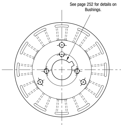
ARMATURE VIEW
