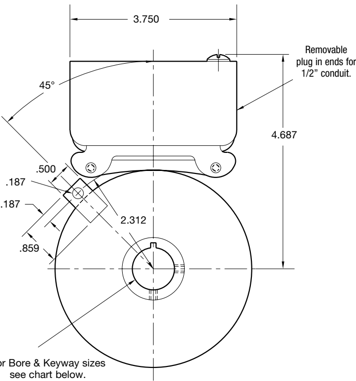
FIELD VIEW
