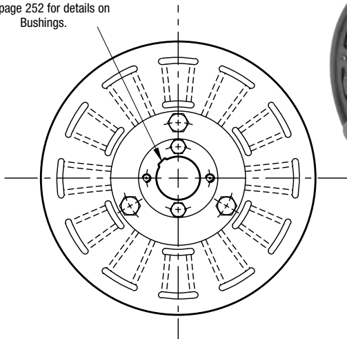
ARMATURE VIEW
