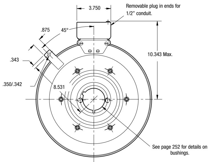
FIELD VIEW
