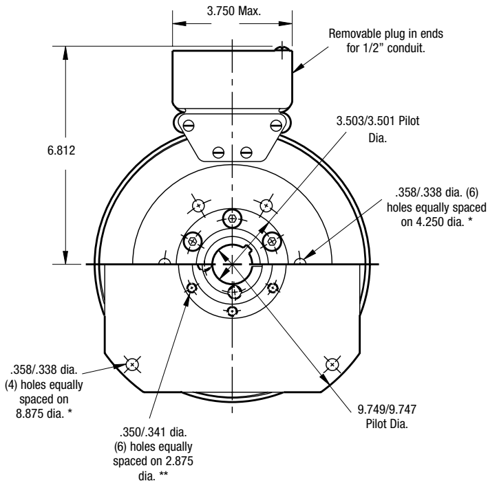
FIELD VIEW
