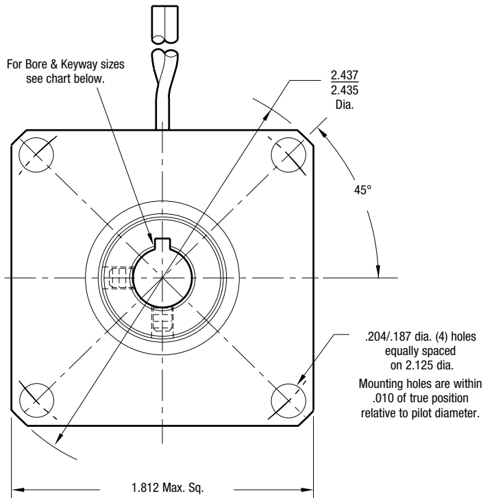
FIELD VIEW
