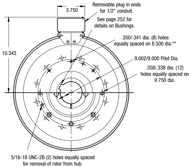
FIELD VIEW
