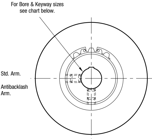
ARMATURE VIEW
