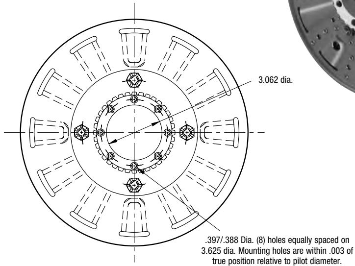
ARMATURE VIEW
