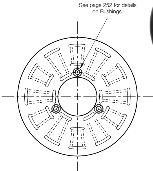
ARMATURE VIEW
