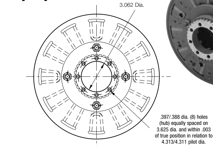
ARMATURE VIEW
