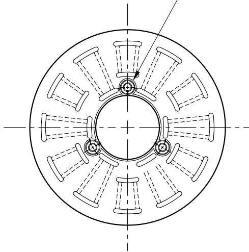
ARMATURE VIEW
