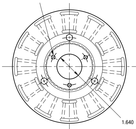
ARMATURE VIEW
