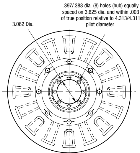
ARMATURE VIEW
